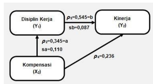
Gambar 5. Diagram Pengaruh X_2 Terhadap Y_2 sab = \sqrt{(b_2sa_2 + a_2sb_2 + sa_2sb_2)}
