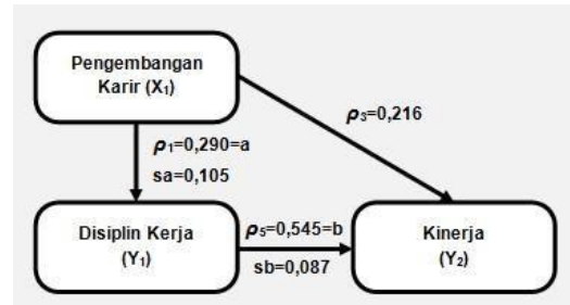
Gambar 4. Diagram Pengaruh X_1 Terhadap Y_2 sab = \sqrt{(b_2sa_2 + a_2sb_2 + sa_2sb_2)}
